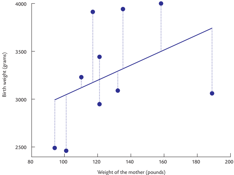
Figure 4.1 Scatter plot of birth weight and weight of the mother with regression line (solid) for ten observations in the LBWS data set. Also shown are vertical lines (dotted) from each observation to the regression line.
