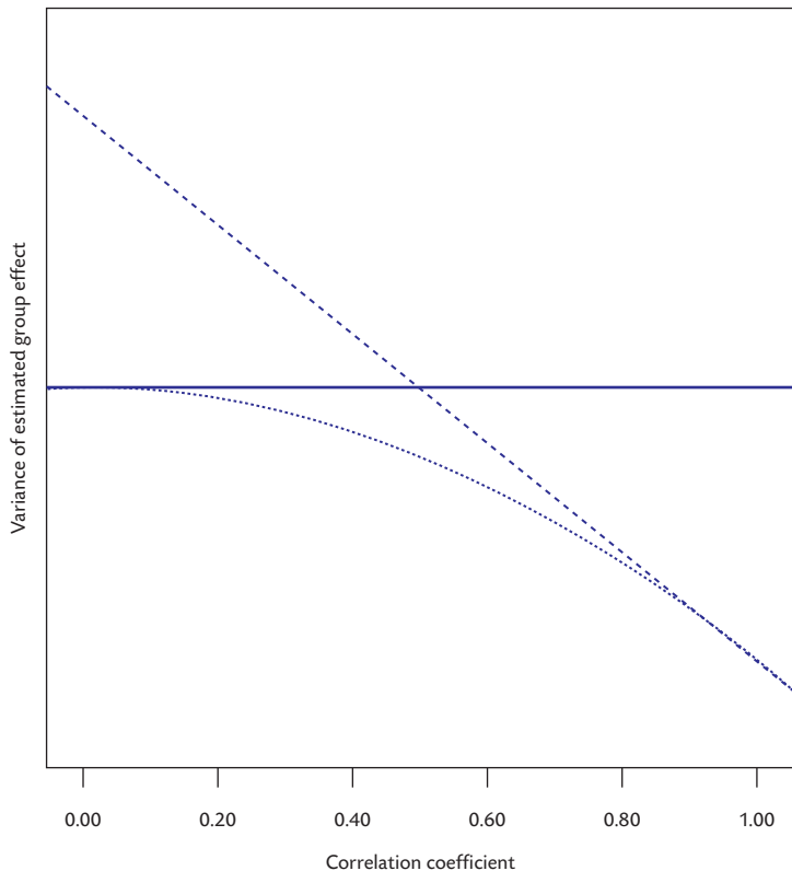
Figure 8.1 The variance of estimated group effects as a function of the correlation between baseline and follow-up measurement for the three approaches described in the text; comparison of follow-up measurement (solid line), comparison of change scores (dashed line), adjustment for baseline (dotted line).
