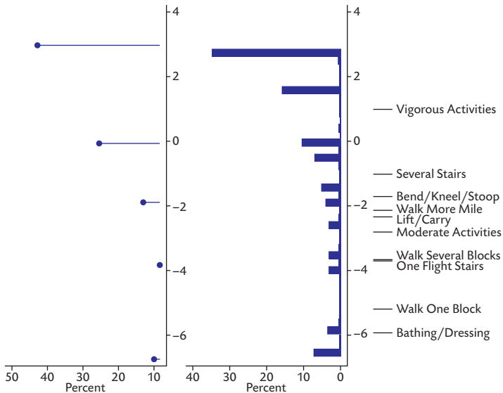
Figure 9.3 Physical functioning. From left to right: Estimated distribution (1-PL with five masspoints), distribution of empirical Bayes scores and difficulties of items. (Source: Rabe-Hesketh and Skrondal, 2008a.)
