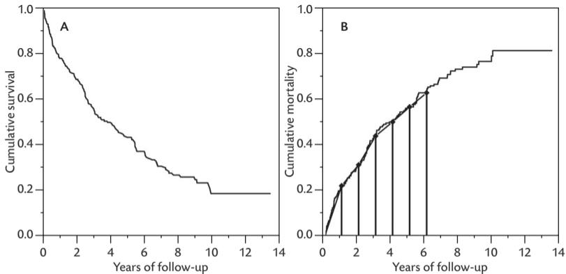
Figure 11.3 A: The survival function S_1 for patients in the placebo arm of the CLS1 trial. B: Cumulative mortality, calculated as P_1 = 1 - S_1 , and a trapezoidal approximation of P_1(6) based on 1-year intervals.
