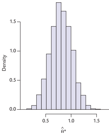
Figure 12.1 Histogram of \hat{\theta}_1^*, \dots, \hat{\theta}_{5000}^* for the CD4 counts data when \hat{\theta} is the median of the change in counts. Left panel: nonparametric bootstrap. Right panel: parametric bootstrap assuming normal distribution.
