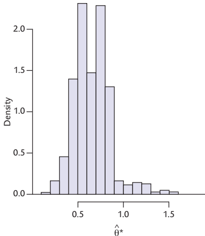
Figure 12.1 Histogram of \hat{\theta}_1^*, \dots, \hat{\theta}_{5000}^* for the CD4 counts data when \hat{\theta} is the median of the change in counts. Left panel: nonparametric bootstrap. Right panel: parametric bootstrap assuming normal distribution.
