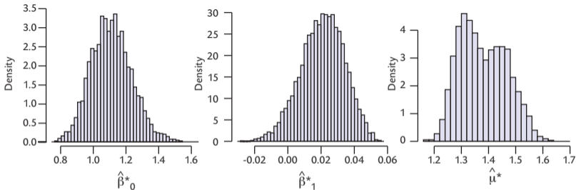
Figure 12.5 Histogram of 5000 simulations of \hat{\beta}_0^* (left), \hat{\beta}_1^* (middle) and \hat{\mu}^* (right) for ordinary regression on the glucose data set.
