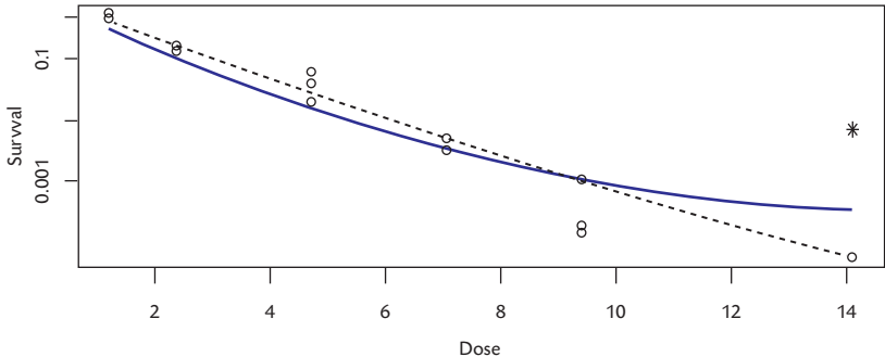
Figure 12.6 Log survival proportion as a function of dose for rats at a succession of doses of radiation (Rads/100). Imposed are LS (solid line) and LAD (dotted line) regression lines.
