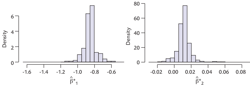
Figure 12.7 Histograms of \hat{\beta}_{m,j}^* for j=1 (left), and j=2 (right). Semi-parametric bootstrap with estimates obtained by the LAD criterion.
