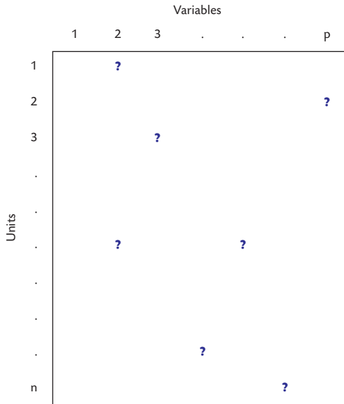
Figure 13.1 Missing data as “holes” in the data matrix.
