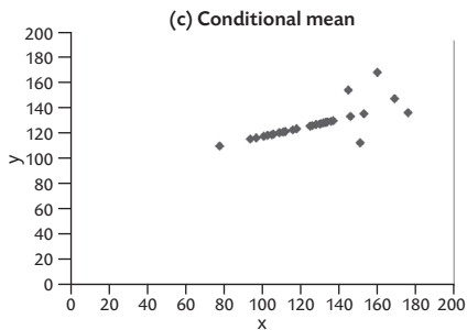
Figure 13.2 Scatter plots of blood pressure measured at two occasions, original data and with missing at random values imputed by three methods.
