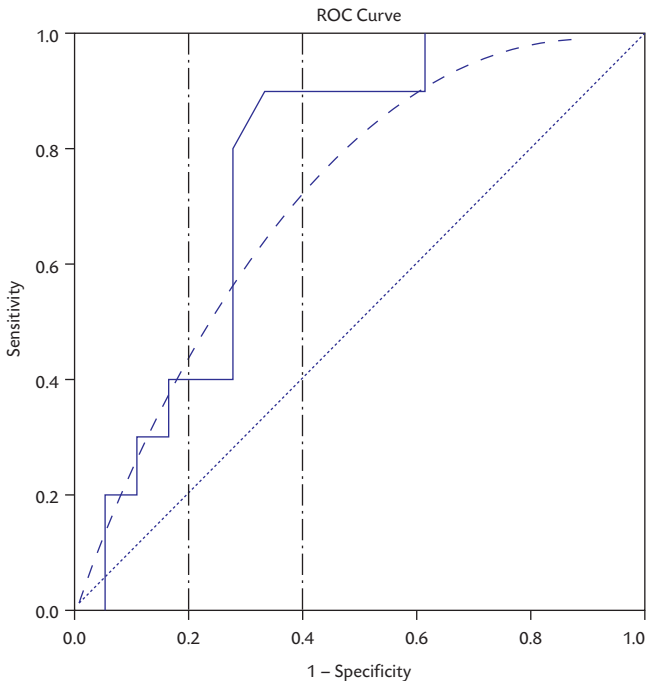
Figure 14.2 Empirical ROC curve (solid line), ROC curve for fitted normal distributions (dashed line), and ROC curve for a non-informative test (dotted line). The partial area under the ROC curve between 1 - \text{Specificity} for e_1 = 0.2 and e_2 = 0.4 is taken between the dash-dot lines.
