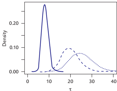
Figure 17.3 On the left, prior densities for \tau for (a,b) equal to (9,3) (solid line), (0.9,0.3) (dashed line) and (0.09,0.03) (dotted line). On the right, corresponding posterior distributions.
