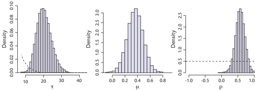
Figure 17.4 Histogram of 100,000 samples from the posterior distribution of \tau, \mu and \rho using prior parameters (a, b) = (0.9, 0.3) . The prior distributions for \tau and \rho are superimposed on the histograms (dashed line).
