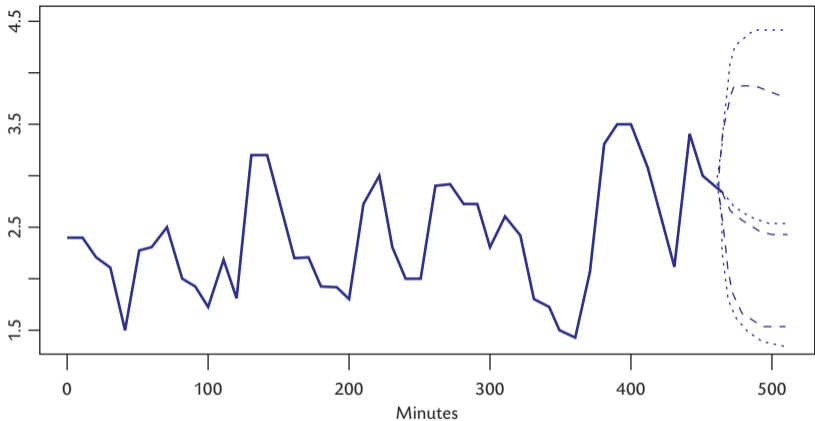
Figure 17.6 Predictions of \exp(Y_{n+k}) for k = 1, 2, 3, 4 . Dashed lines are predictions and 95% prediction intervals for the plug-in rule. Dotted lines are the same quantities for Bayesian prediction using prior parameters a = 0.9 , b = 0.3 .
