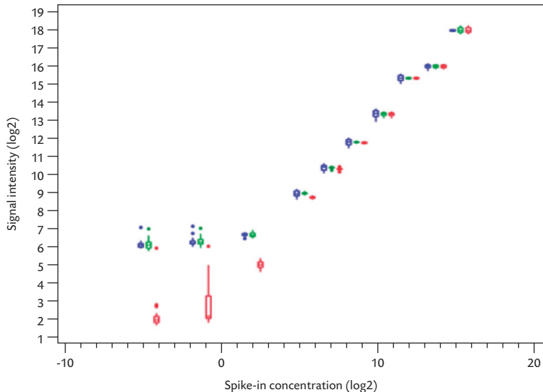
Figure 19.2 Probe intensity as a function of target sequence concentration before and after background correction. The horizontal axis represents the concentration of the target molecules for a collection of spike-in probes in an Agilent gene expression array. The vertical axis represents the measured signal intensity: raw signal (blue), signal corrected for spatial variation (green), and signal corrected for spatial variation and background noise (red).
