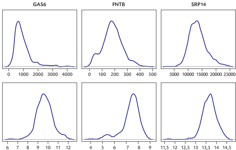
Figure 19.3 Effect of logarithmic transformation on signal intensity distribution. Intensity distributions are shown for three genes (GAS6, FNTB, and SRP14) before logarithmic transformation (top row) and after logarithmic transformation (bottom row). Data are from Affymetrix single-colour gene expression arrays.
